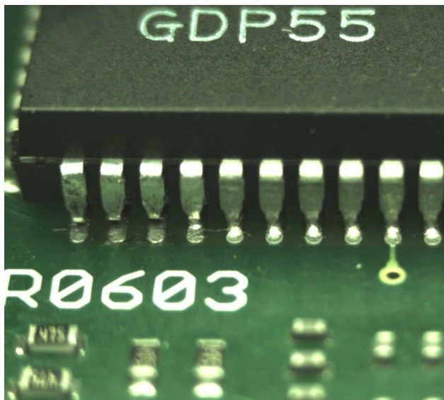
Picture: inspection with angled-view module from S&K
